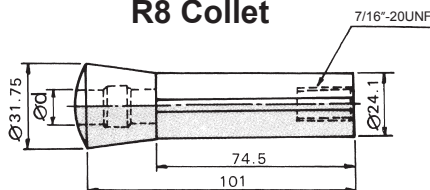
R8 Collet
