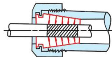
single-taper chuck
