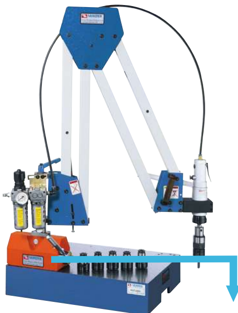
MAGNETIC BASE
