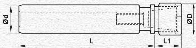
FIG. 1 : With M Type Nut
