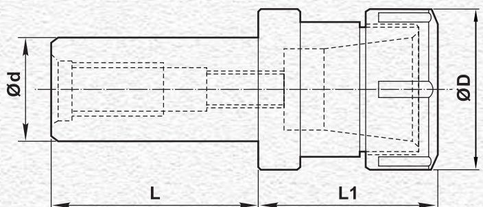
FIG. 3 : With Round Type Nut
