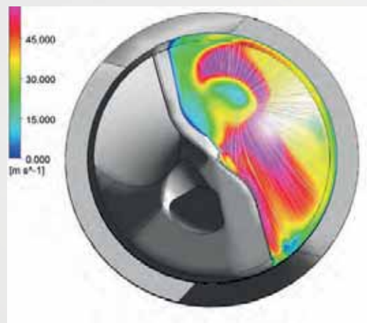
Trigon coolant duct design
