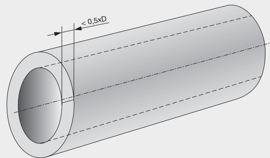
Minimum distance ( 0.5xD ) falling short → can lead to losses in hole straightness
